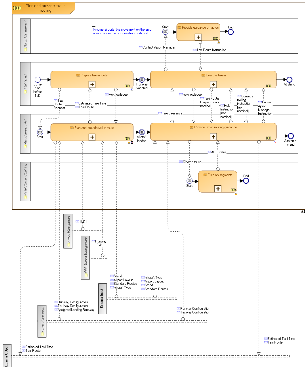
Figure 3: Plan and provide taxi-in routing high-level process
