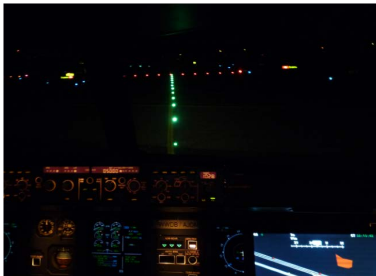
Figure 38: Activated stop bar with TCLs used for individual guidance in the foreground
