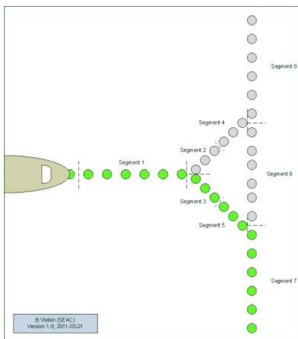
Figure 36: Example for AGL Segments in Phase 1
